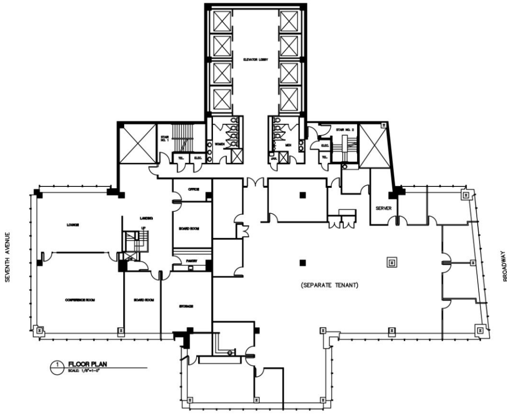
22ND FLOOR PLAN AND REFLECTED CEILING PLAN
