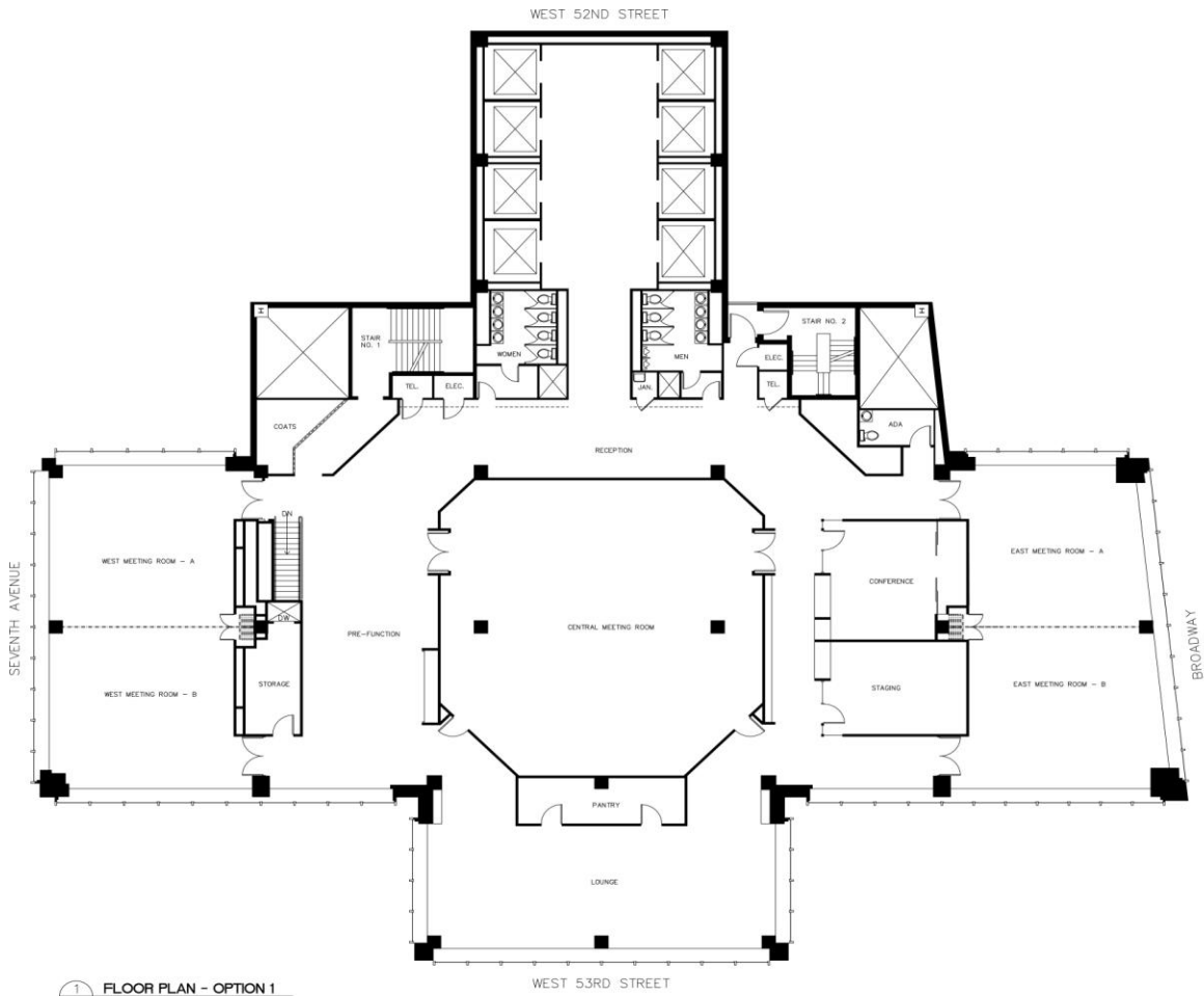
1 FLOOR PLAN - OPTION 1 SCALE: 1/8"=1'-0"
